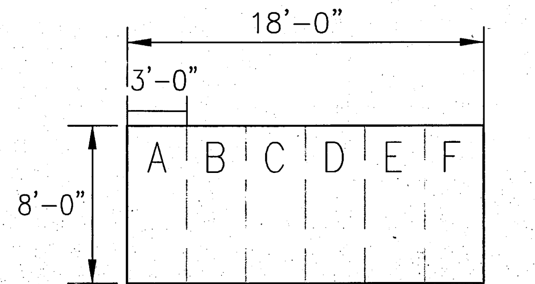
ADULT LAWN CRYPTS PLOT LAYOUT SCALE: 1" = 5'
